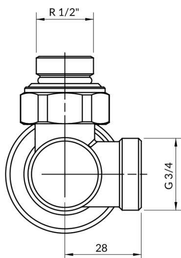
Winkel-Thermostatventil
