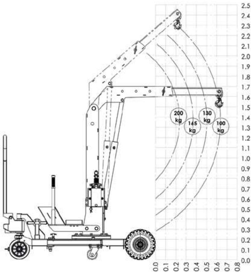
STANDARDARM
