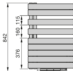
Vista frontale, ROFR-090
