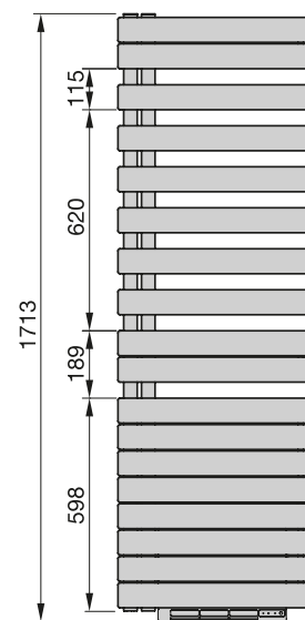
Vista frontale, ROFR-180
