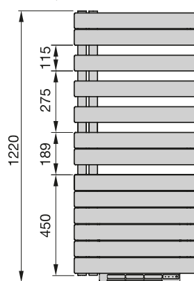
Vista frontale, ROFR-130
